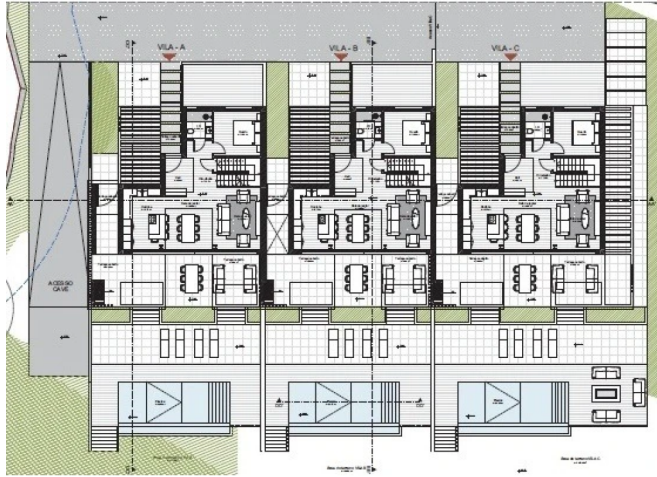
Ground Floor Plans
