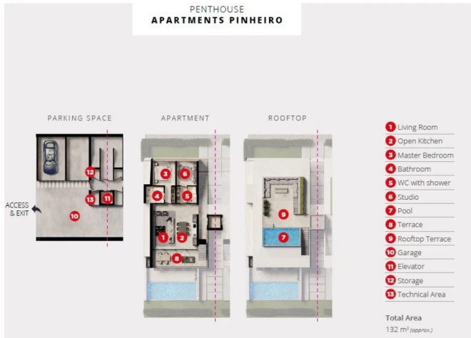
Penthouse Floor Plan
