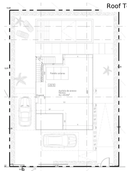
Roof Terrace Plan
